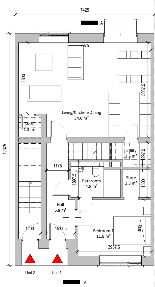
① Ground Floor - Mid Terrace 1 : 100
