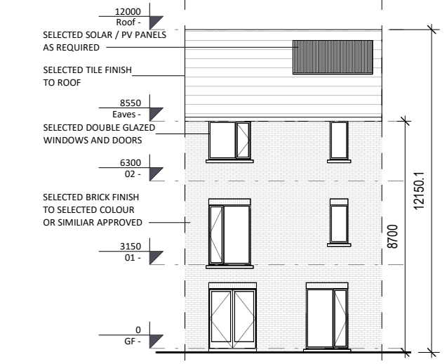
⑤ Rear Elevation - Mid Terrace 1 : 200
