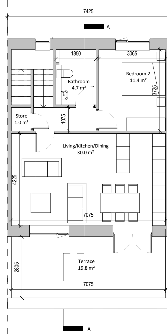
③ Second Floor - Mid Terrace 1 : 100
