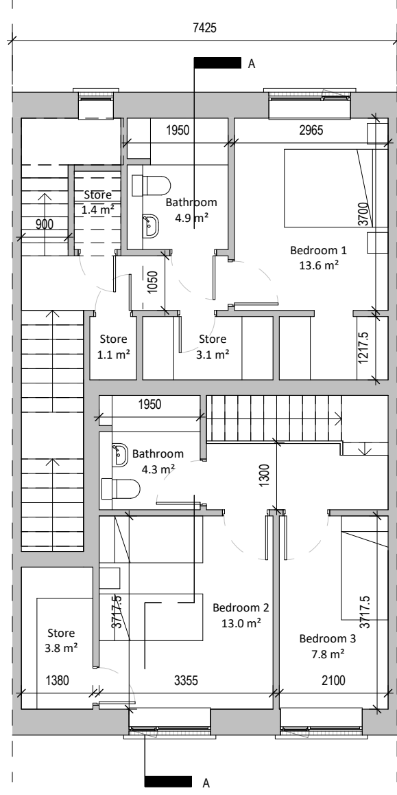
② First Floor - Mid Terrace 1 : 100
